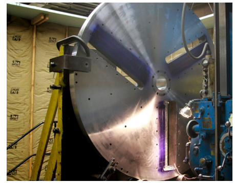
Each disc is fabricated from plate steel and put through ultrasonic testing, and material certified.
