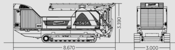
Transport position
