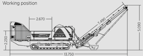
Working position
