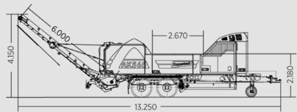
Working position
