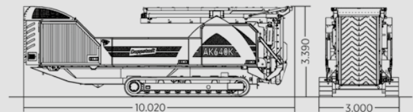
Transport position
