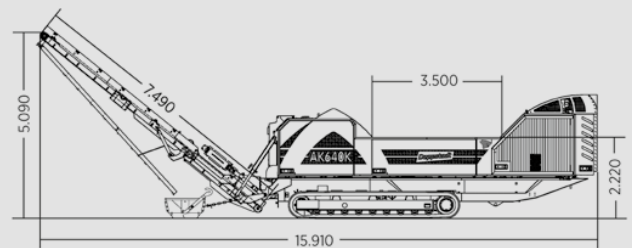
Working position
